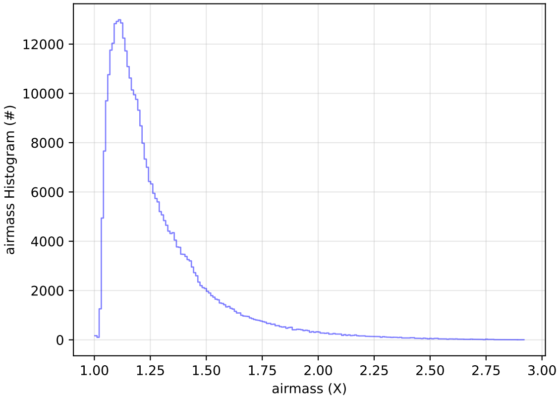
too_elab_r128_d3_gz_v3.4_10yrs WFD y band: airmass Histogram
