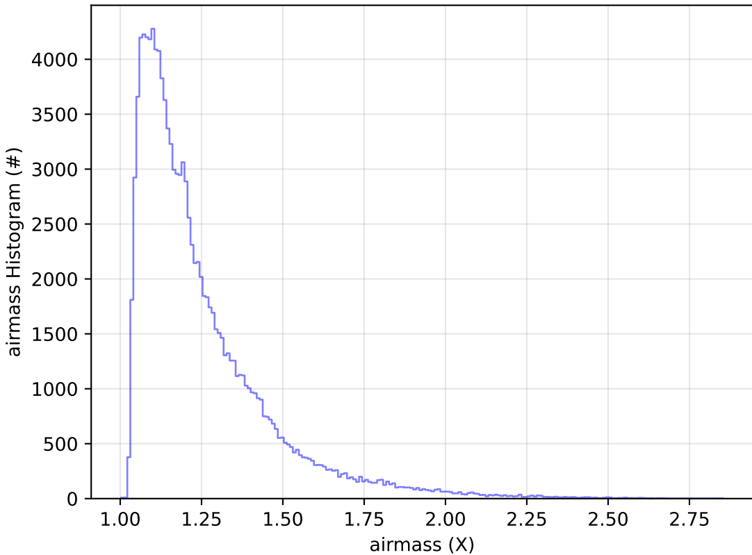
too_elab_r128_d3_gz_v3.4_10yrs WFD u band: airmass Histogram
