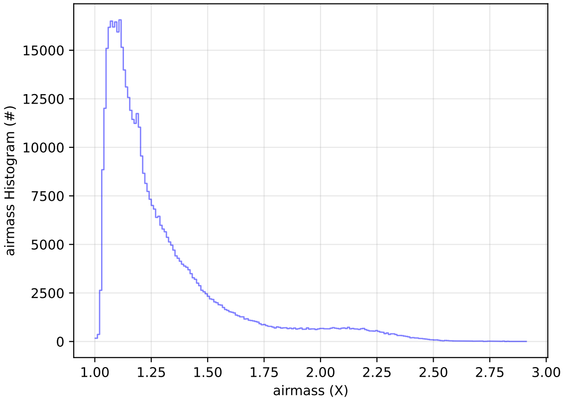
too_elab_r128_d3_gz_v3.4_10yrs WFD r band: airmass Histogram
