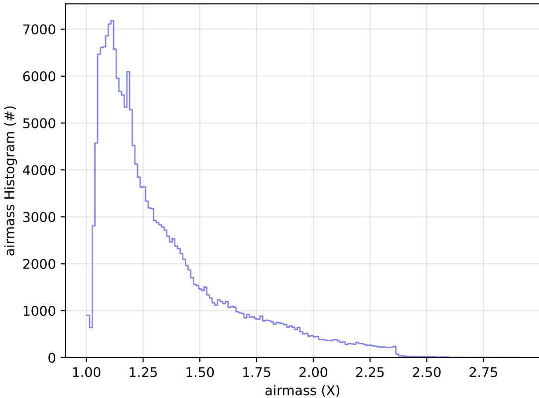
too_elab_r128_d3_gz_v3.4_10yrs WFD g band: airmass Histogram
