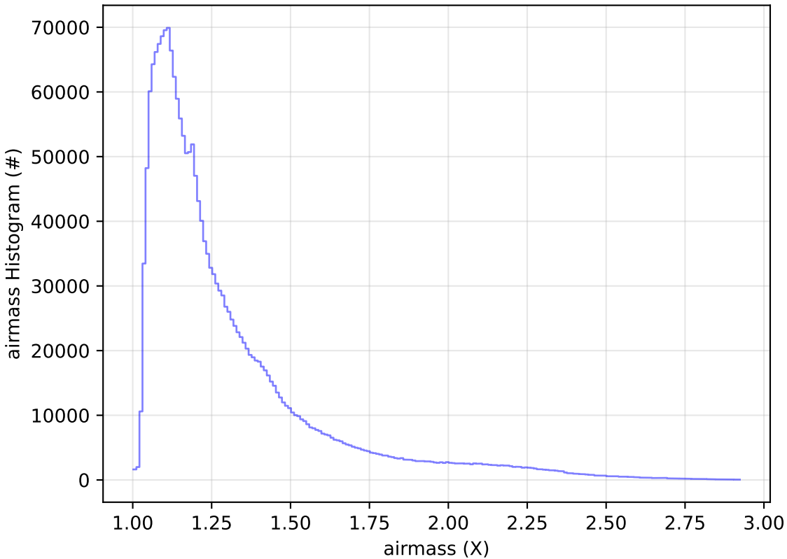
too_elab_r128_d3_gz_v3.4_10yrs WFD all bands: airmass Histogram
