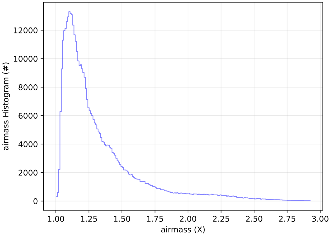
too_elab_r128_d3_gz_v3.4_10yrs All sky z band: airmass Histogram
