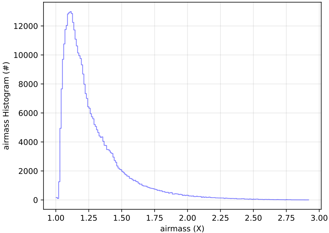
too_elab_r128_d3_gz_v3.4_10yrs All sky y band: airmass Histogram
