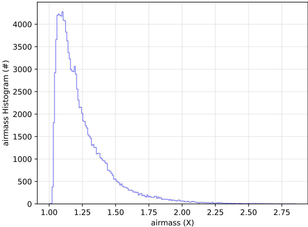
too_elab_r128_d3_gz_v3.4_10yrs All sky u band: airmass Histogram
