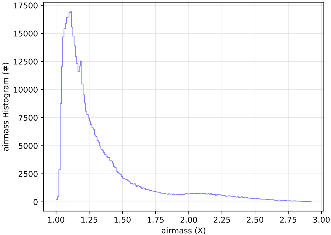
too_elab_r128_d3_gz_v3.4_10yrs All sky i band: airmass Histogram
