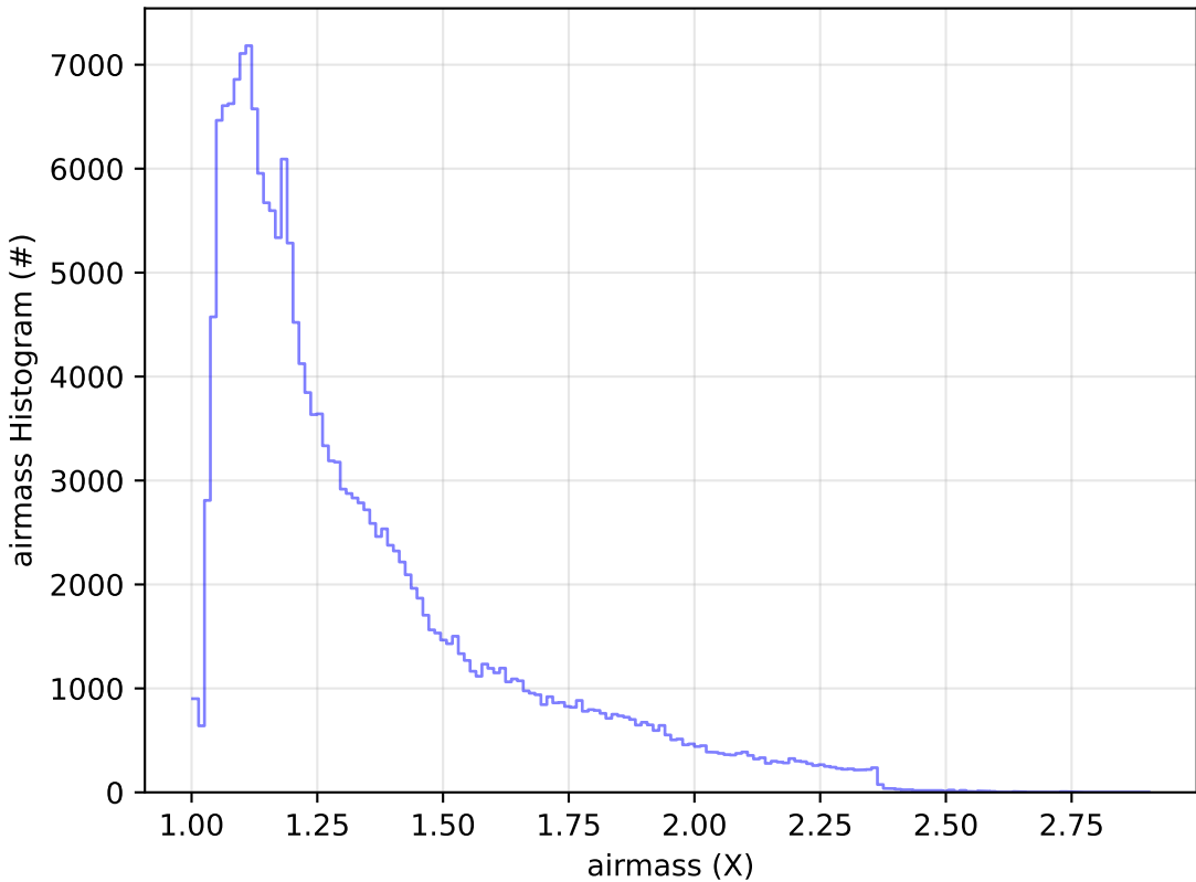
too_elab_r128_d3_gz_v3.4_10yrs All sky g band: airmass Histogram
