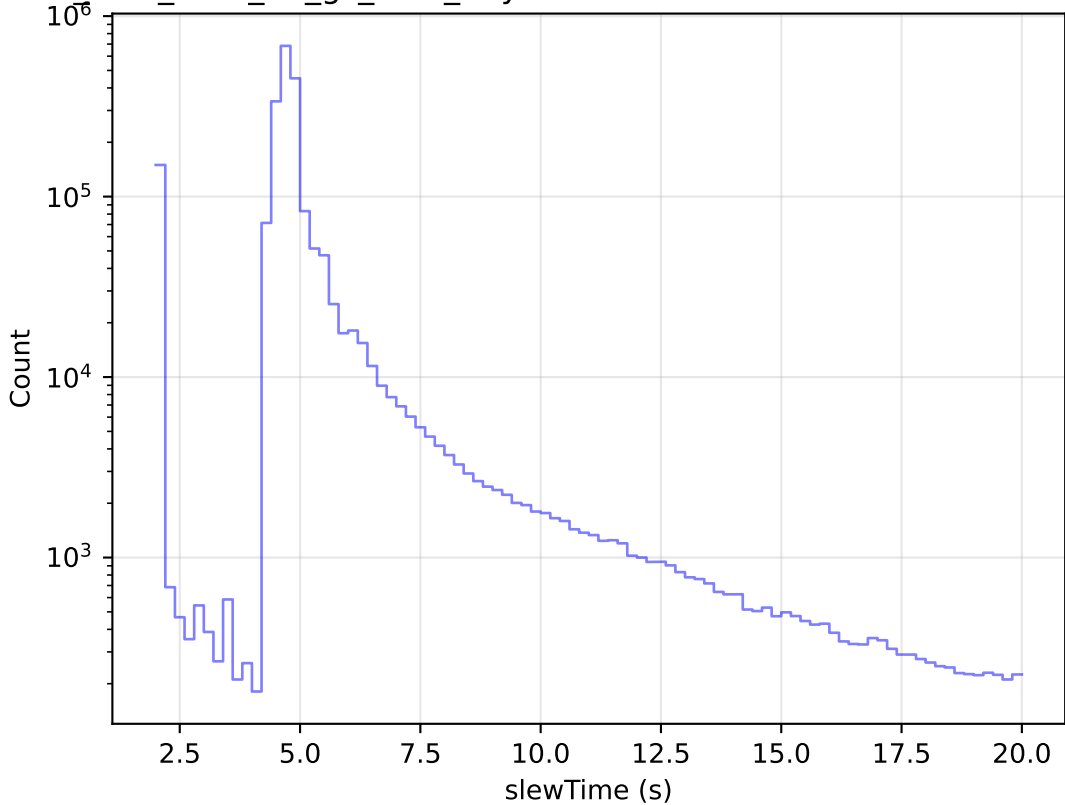
too_elab_r128_d3_gz_v3.4_10yrs All visits: Zoom Slew Time Histogram
