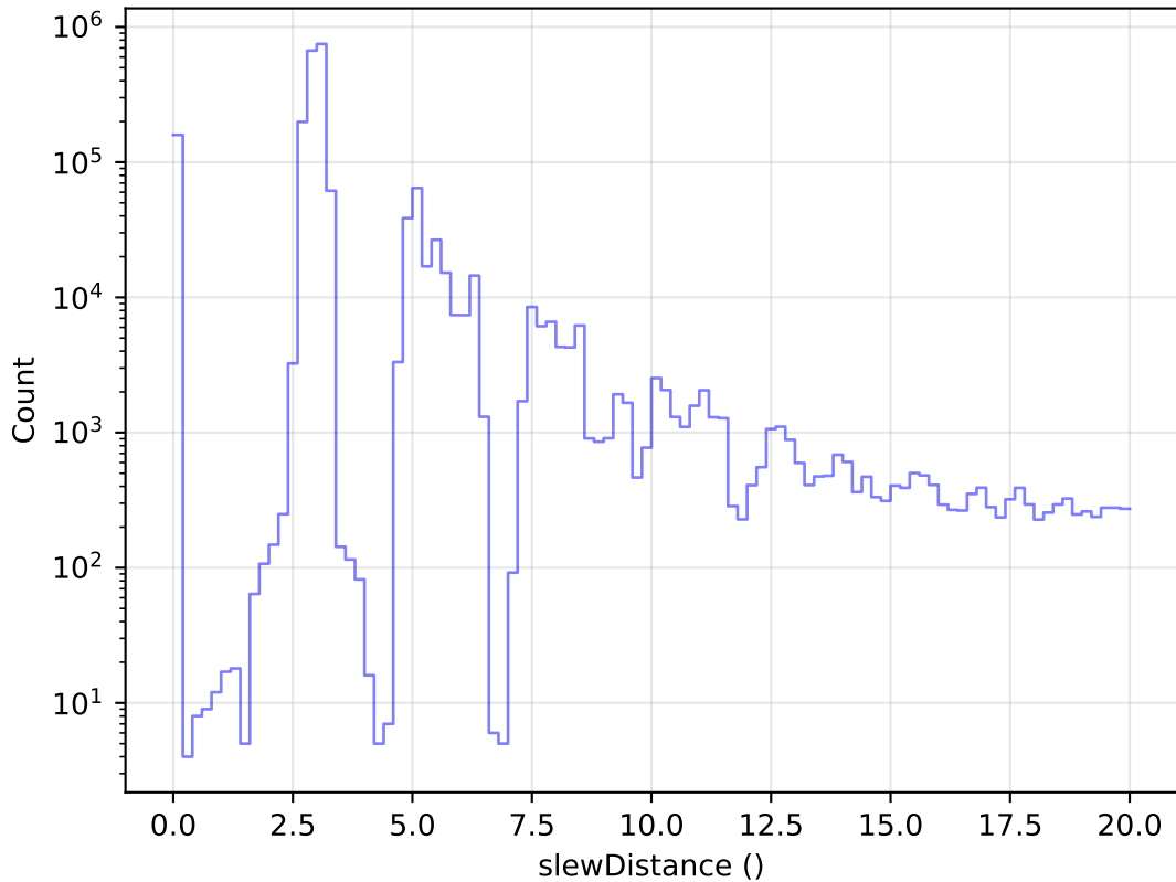
too_elab_r128_d3_gz_v3.4_10yrs All visits: Zoom Slew Distance Histogram
