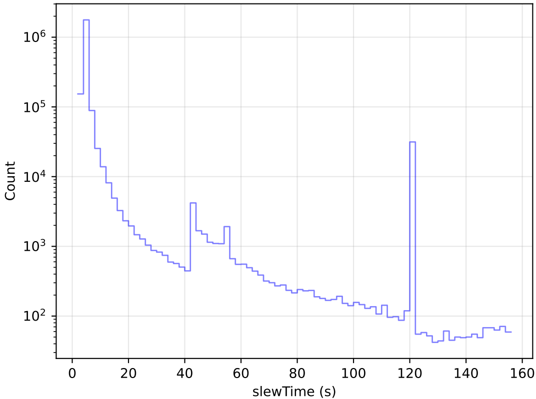
too_elab_r128_d3_gz_v3.4_10yrs All visits: Slew Time Histogram
