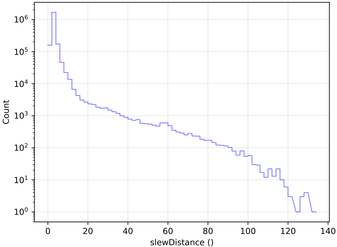
too_elab_r128_d3_gz_v3.4_10yrs All visits: Slew Distance Histogram
