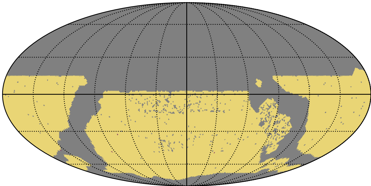
too_elab_r128_d3_gz_v3.4_10yrs WFD: RapidRevisits
