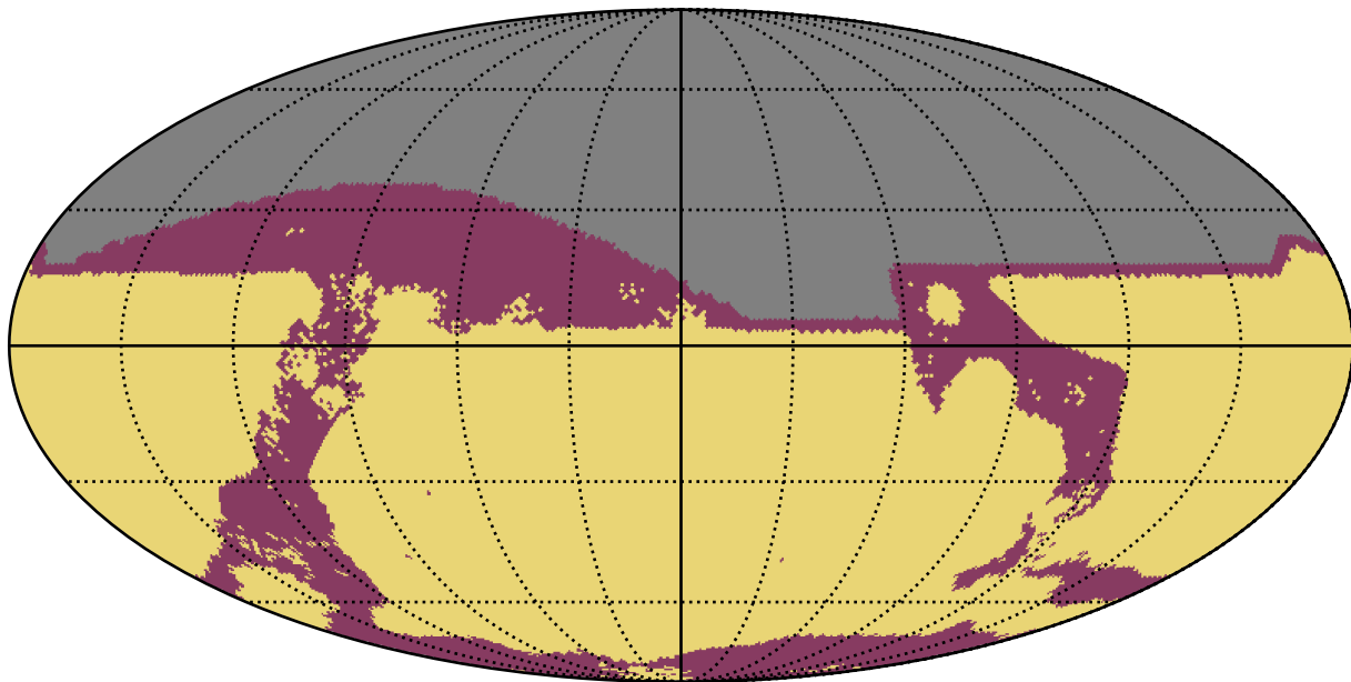
too_elab_r128_d3_gz_v3.4_10yrs All sky: RapidRevisits
