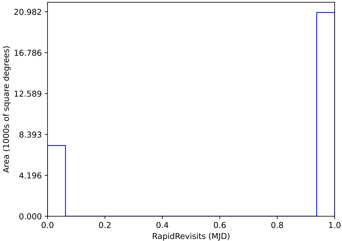
too_elab_r128_d3_gz_v3.4_10yrs All sky: RapidRevisits
