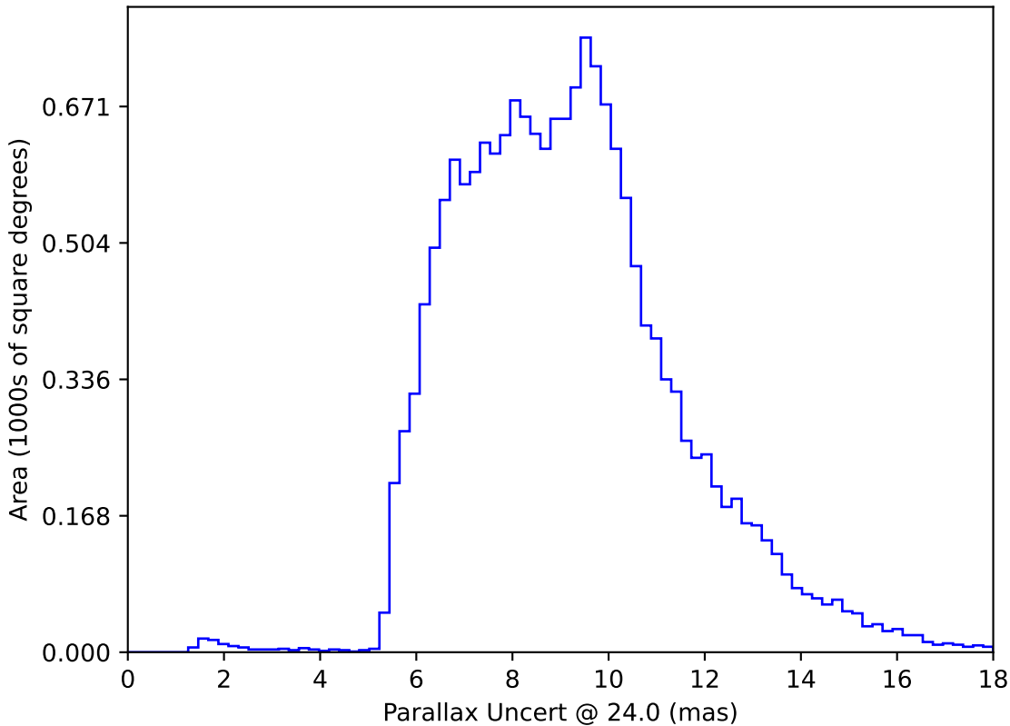
too_elab_r128_d3_gz_v3.4_10yrs WFD: Parallax Uncert @ 24.0
