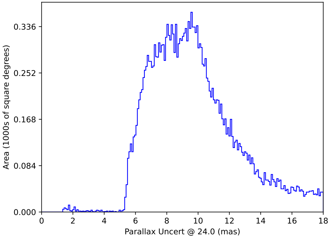
too_elab_r128_d3_gz_v3.4_10yrs All sky: Parallax Uncert @ 24.0
