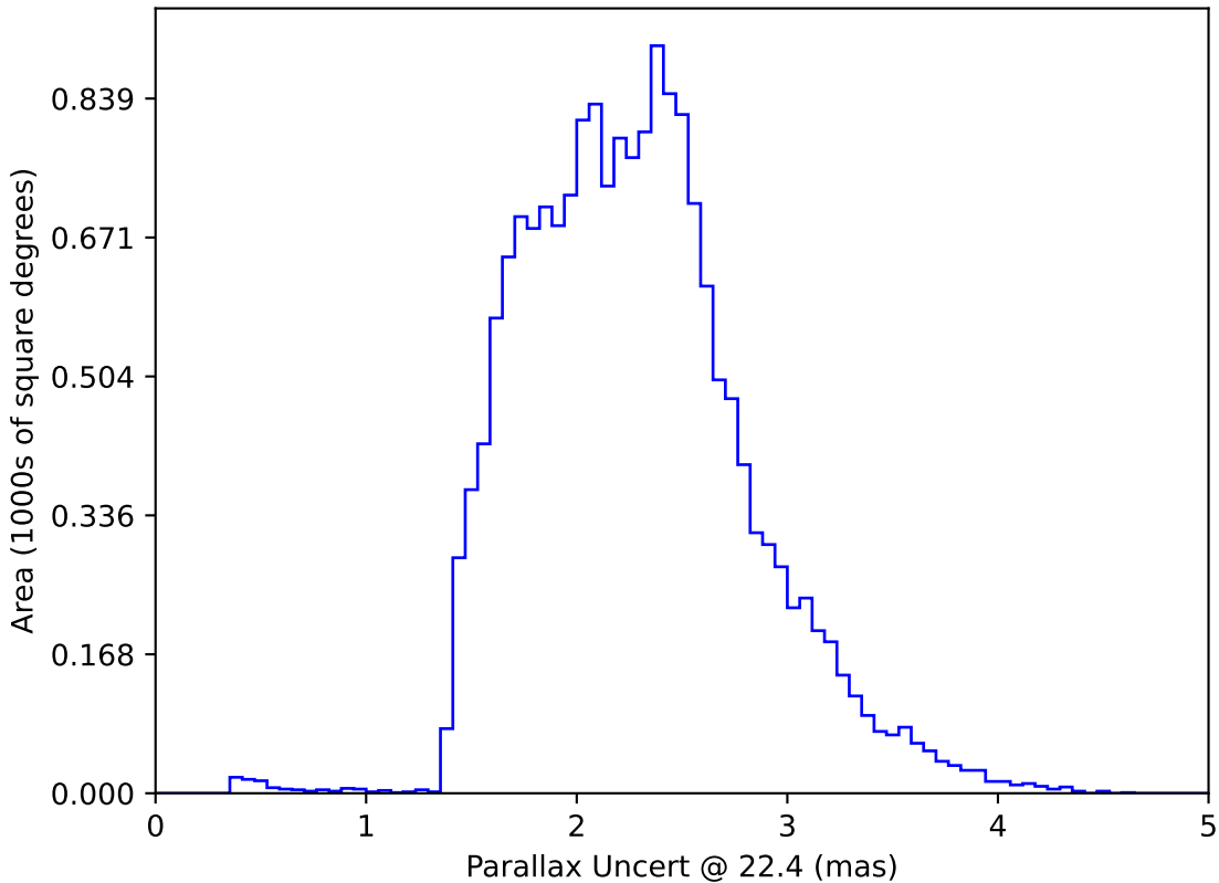
too_elab_r128_d3_gz_v3.4_10yrs WFD: Parallax Uncert @ 22.4
