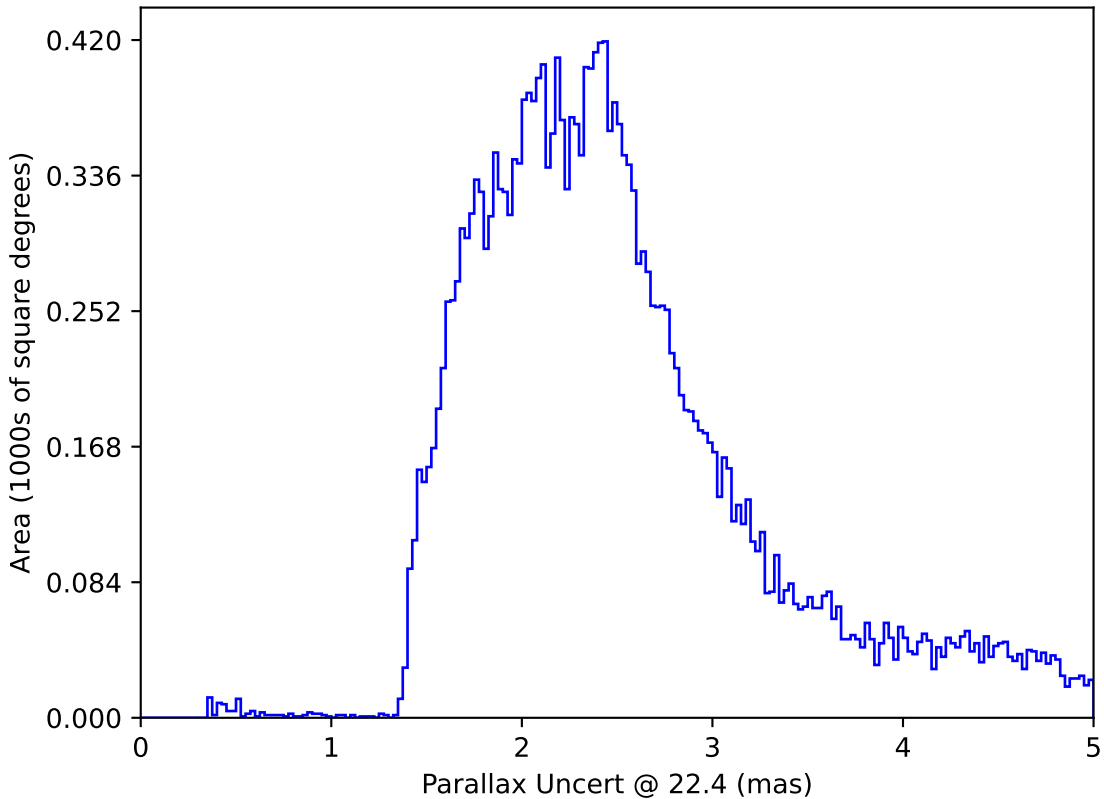
too_elab_r128_d3_gz_v3.4_10yrs All sky: Parallax Uncert @ 22.4
