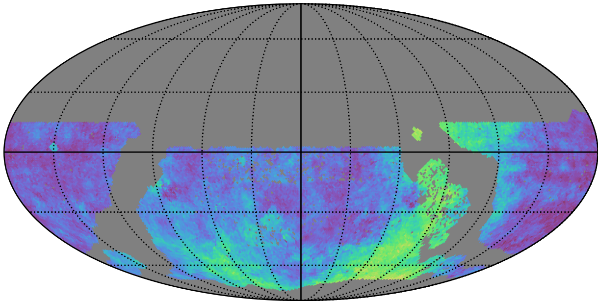
too_elab_r128_d3_gz_v3.4_10yrs WFD: Parallax Coverage @ 24.0
