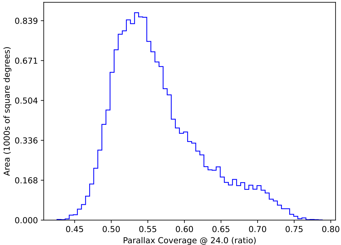
too_elab_r128_d3_gz_v3.4_10yrs WFD: Parallax Coverage @ 24.0
