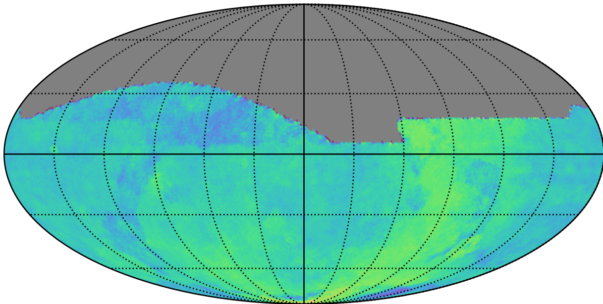
too_elab_r128_d3_gz_v3.4_10yrs All sky: Parallax Coverage @ 24.0
