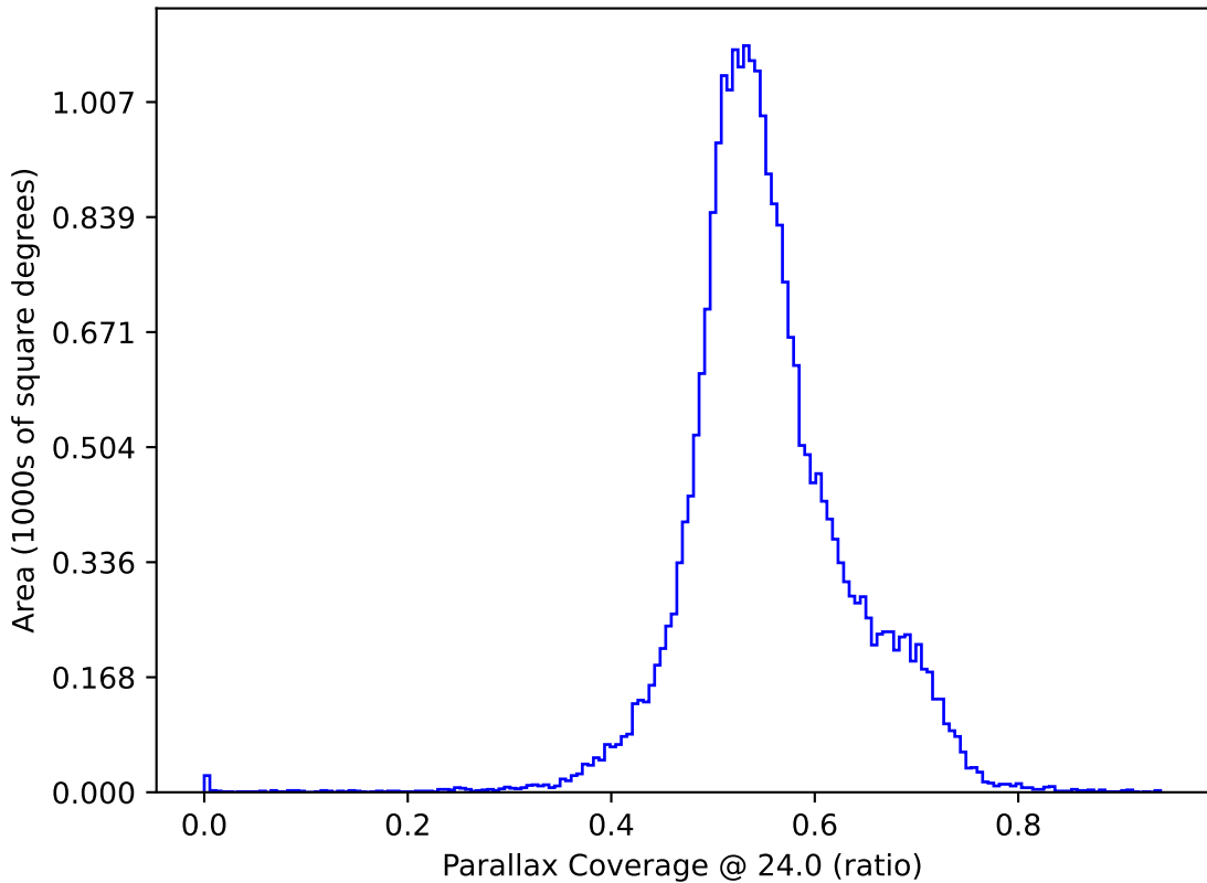
too_elab_r128_d3_gz_v3.4_10yrs All sky: Parallax Coverage @ 24.0
