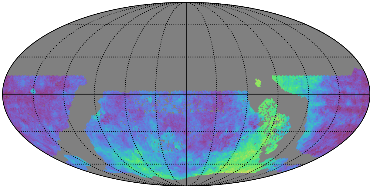
too_elab_r128_d3_gz_v3.4_10yrs WFD: Parallax Coverage @ 22.4
