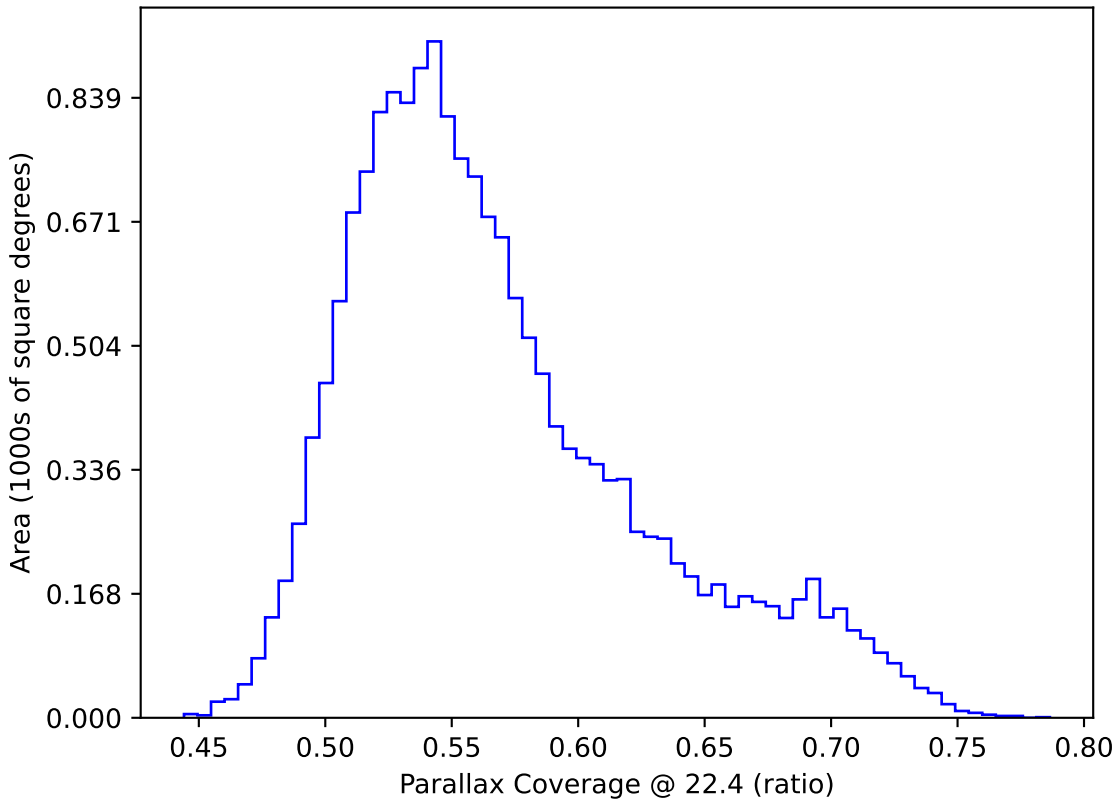
too_elab_r128_d3_gz_v3.4_10yrs WFD: Parallax Coverage @ 22.4
