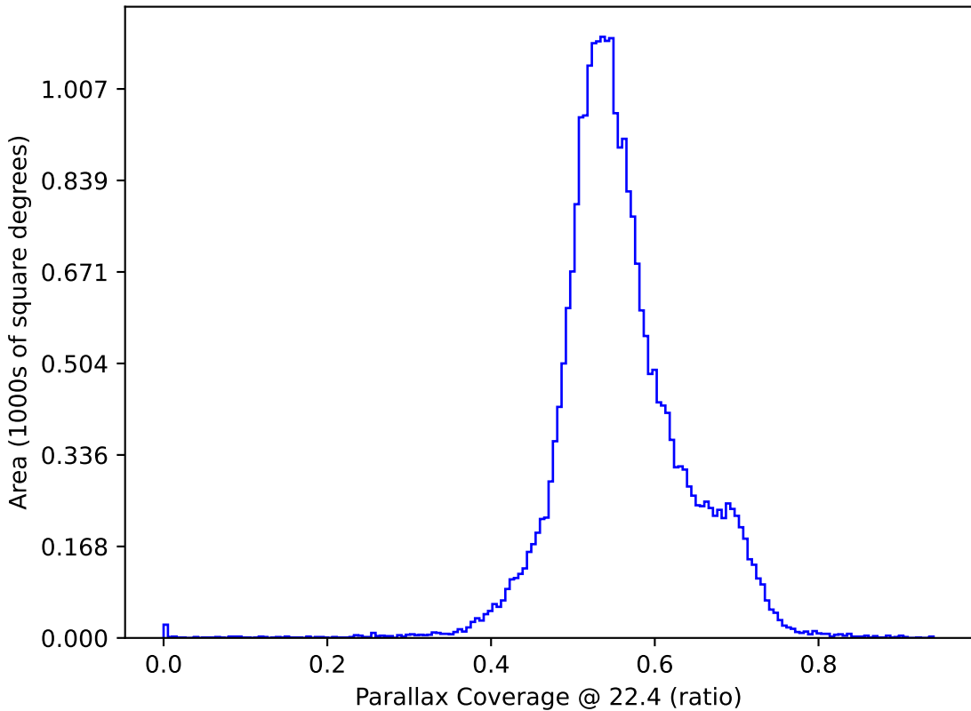
too_elab_r128_d3_gz_v3.4_10yrs All sky: Parallax Coverage @ 22.4
