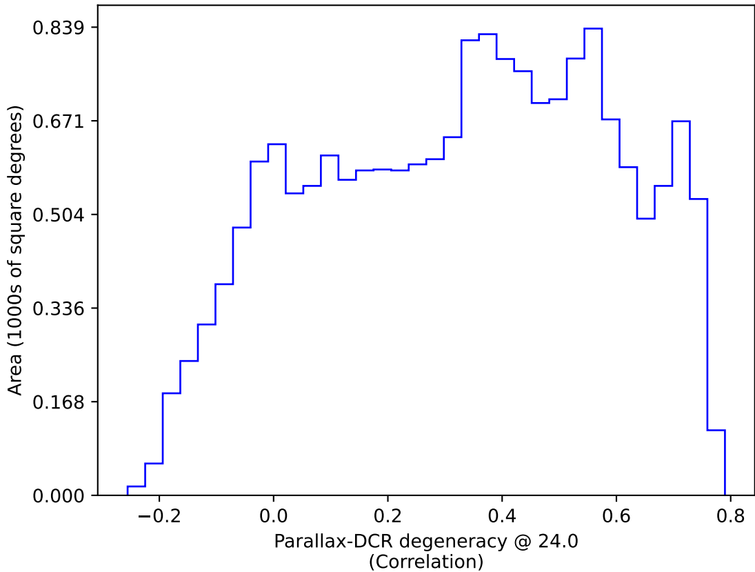
too_elab_r128_d3_gz_v3.4_10yrs WFD: Parallax-DCR degeneracy @ 24.0
