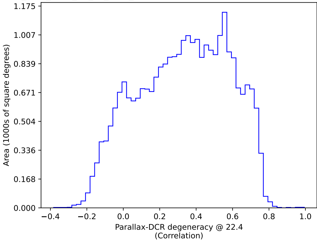
too_elab_r128_d3_gz_v3.4_10yrs All sky: Parallax-DCR degeneracy @ 22.4
