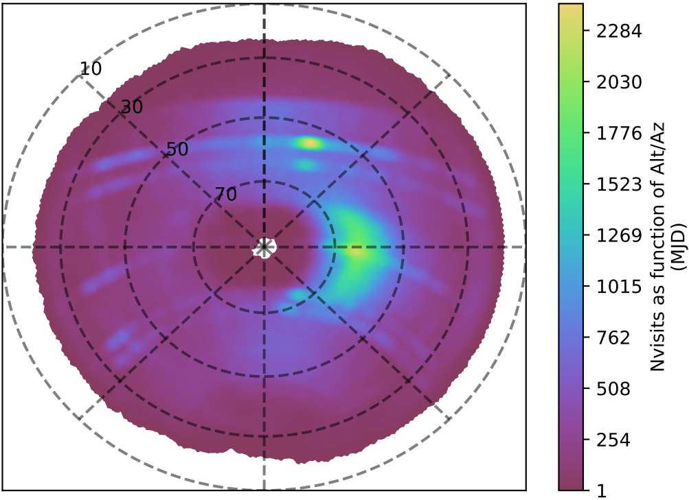
too_elab_r128_d3_gz_v3.4_10yrs z band: Nvisits as function of Alt/Az
