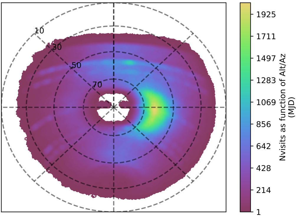
too_elab_r128_d3_gz_v3.4_10yrs y band: Nvisits as function of Alt/Az
