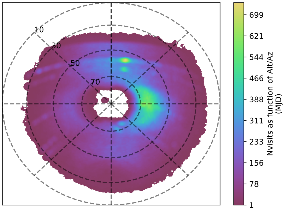
too_elab_r128_d3_gz_v3.4_10yrs u band: Nvisits as function of Alt/Az
