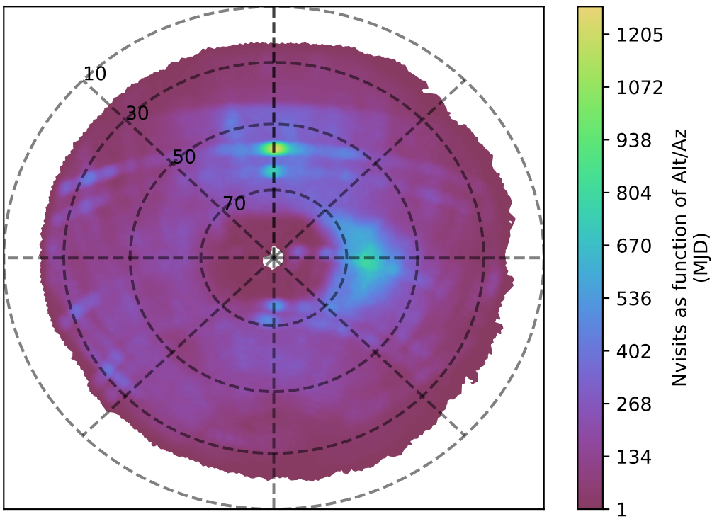
too_elab_r128_d3_gz_v3.4_10yrs g band: Nvisits as function of Alt/Az
