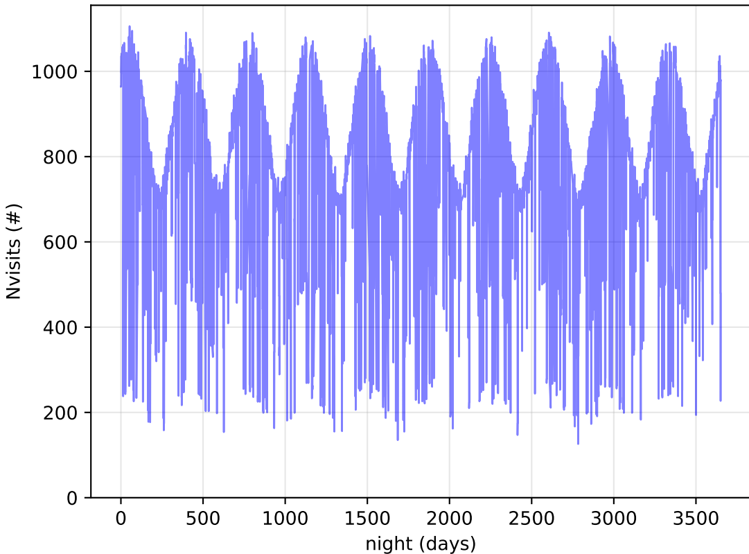
too_elab_r128_d3_gz_v3.4_10yrs All visits: Nvisits
