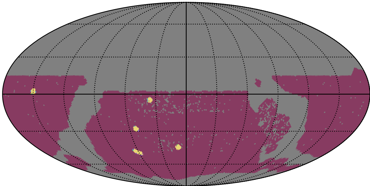
too_elab_r128_d3_gz_v3.4_10yrs WFD: NumberOfQuickRevisits
