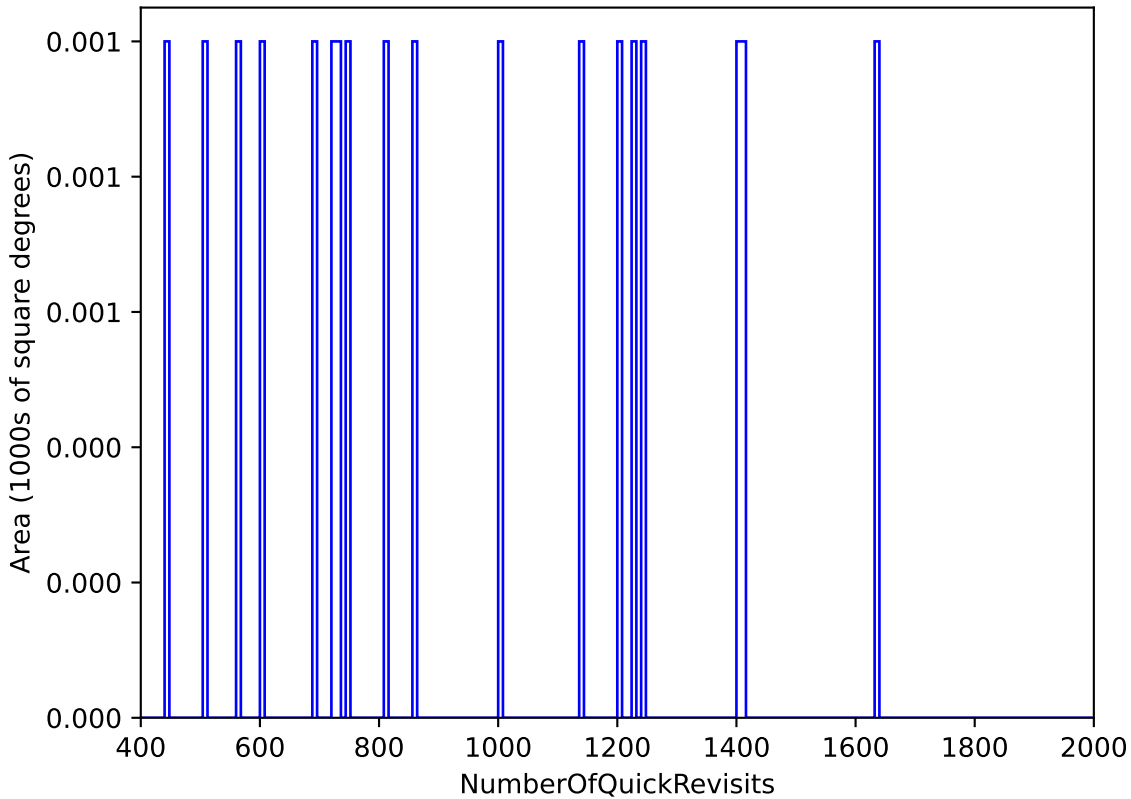
too_elab_r128_d3_gz_v3.4_10yrs WFD: NumberOfQuickRevisits
