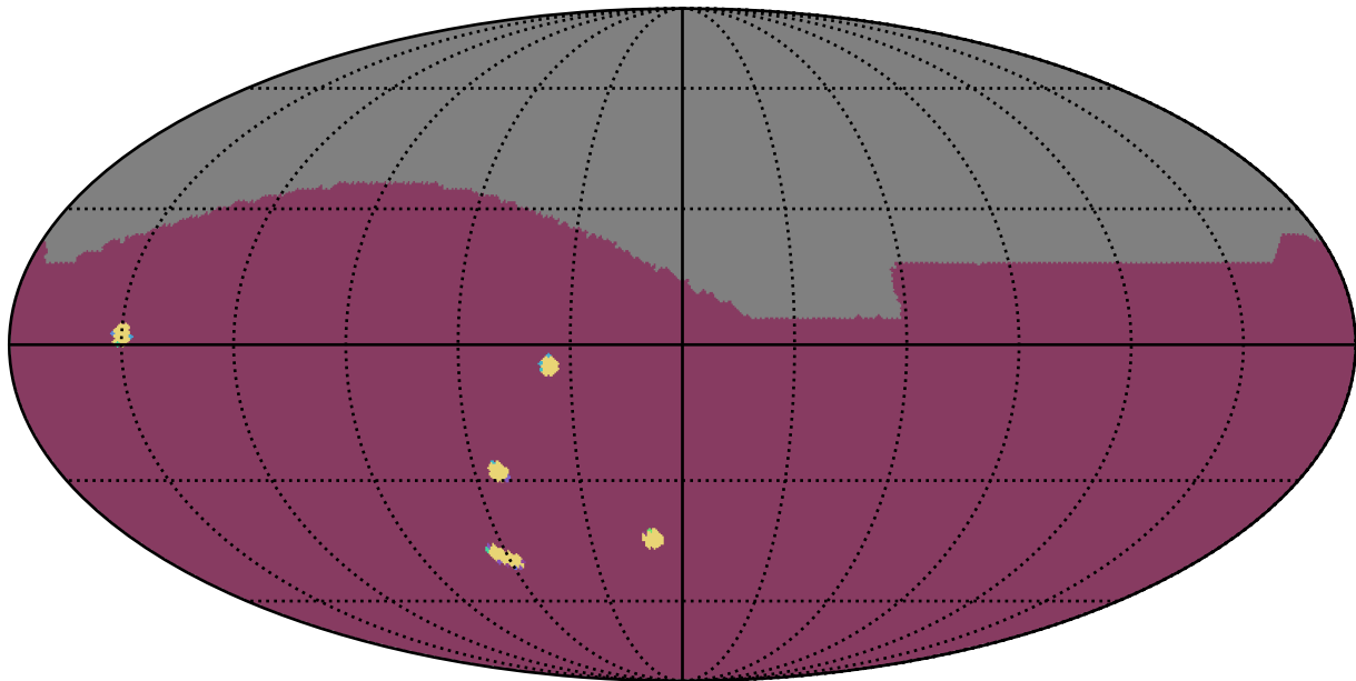
too_elab_r128_d3_gz_v3.4_10yrs All sky: NumberOfQuickRevisits
