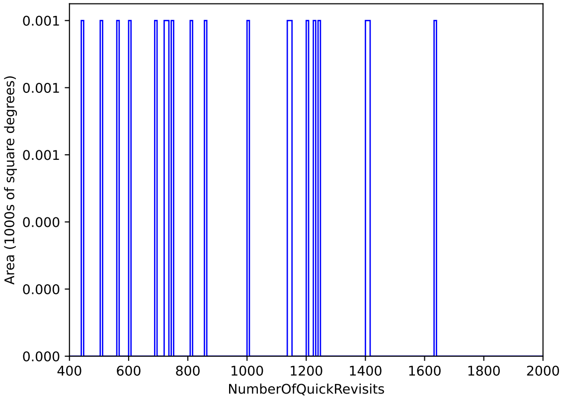
too_elab_r128_d3_gz_v3.4_10yrs All sky: NumberOfQuickRevisits
