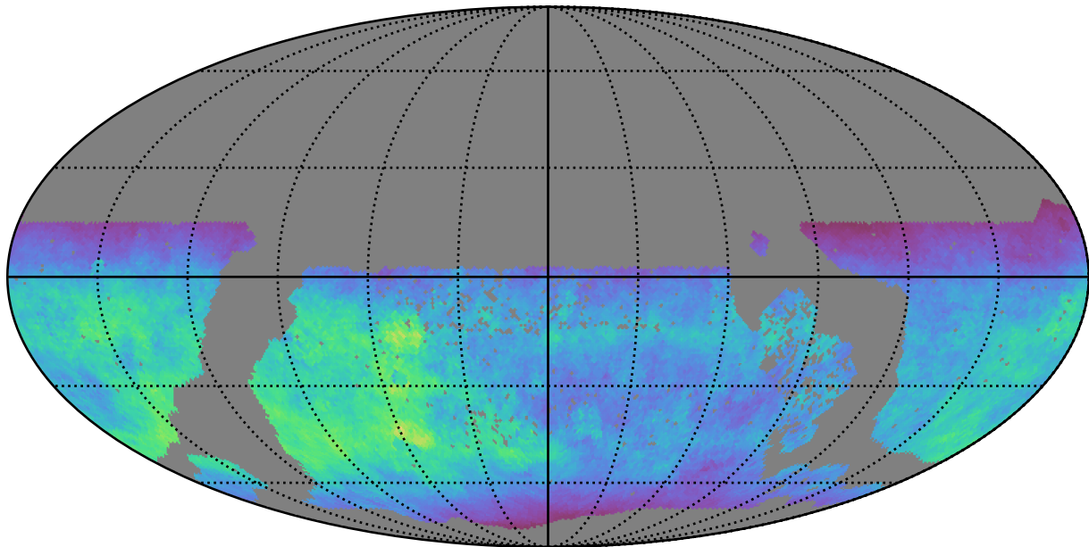
too_elab_r128_d3_gz_v3.4_10yrs WFD z band: Normalized Teff
