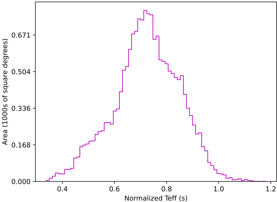
too_elab_r128_d3_gz_v3.4_10yrs WFD z band: Normalized Teff
