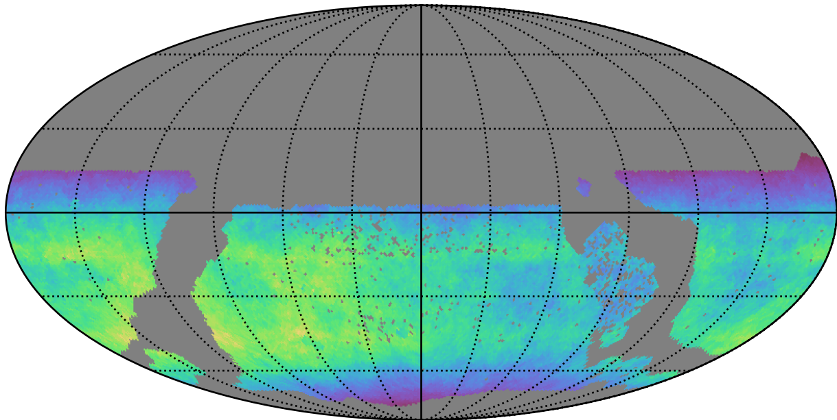
too_elab_r128_d3_gz_v3.4_10yrs WFD y band: Normalized Teff
