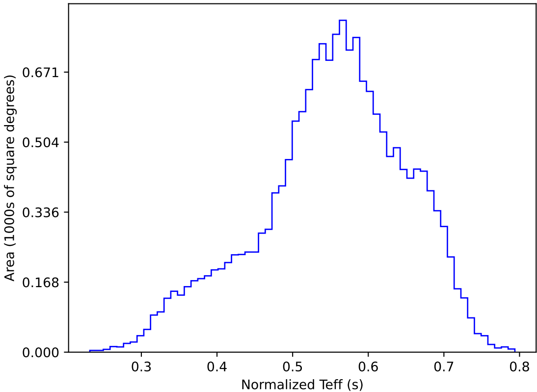
too_elab_r128_d3_gz_v3.4_10yrs WFD y band: Normalized Teff
