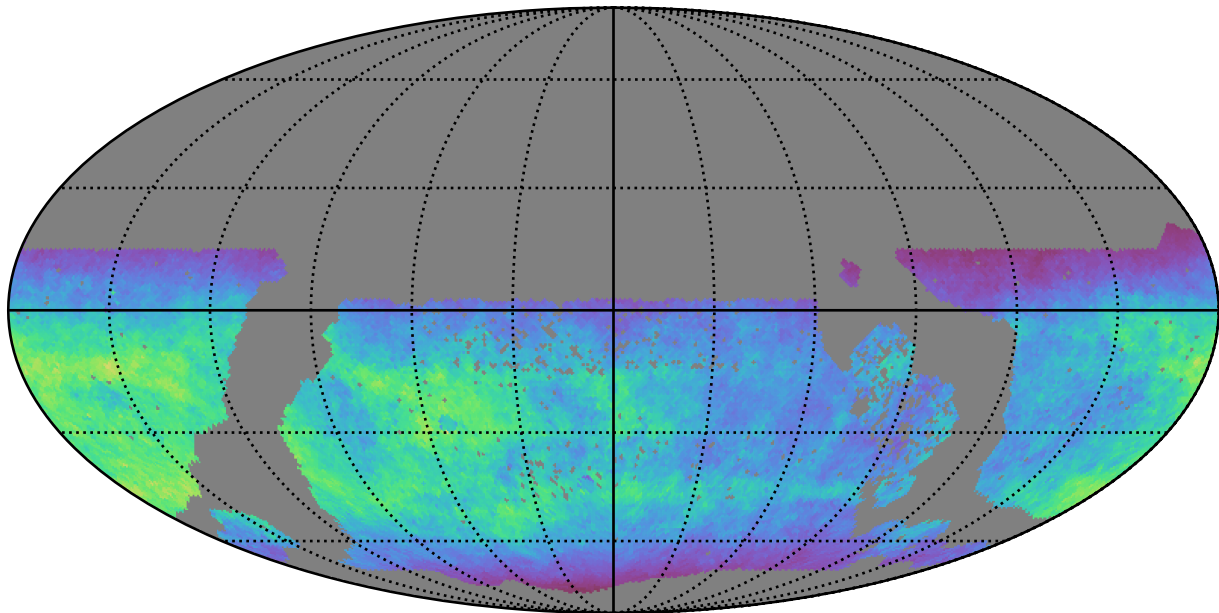
too_elab_r128_d3_gz_v3.4_10yrs WFD u band: Normalized Teff
