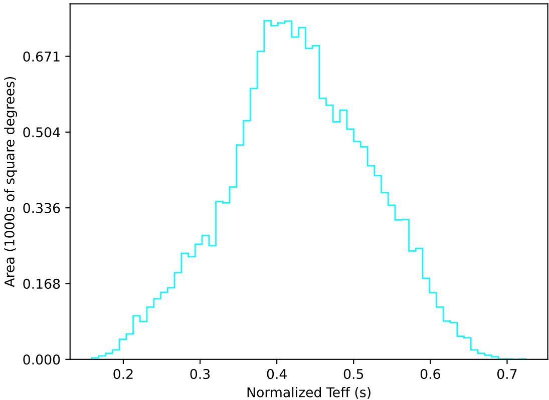
too_elab_r128_d3_gz_v3.4_10yrs WFD u band: Normalized Teff
