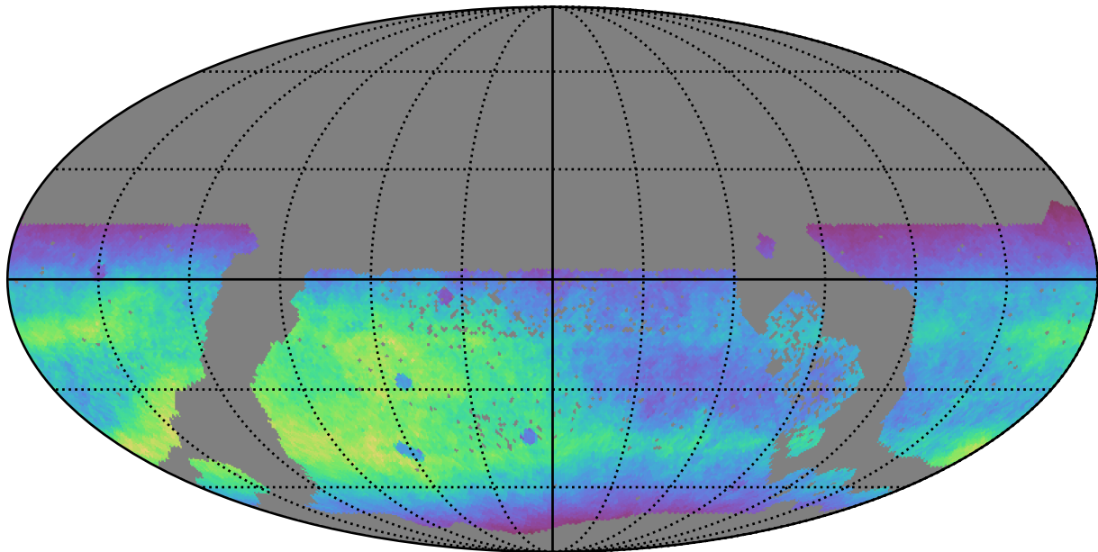
too_elab_r128_d3_gz_v3.4_10yrs WFD r band: Normalized Teff
