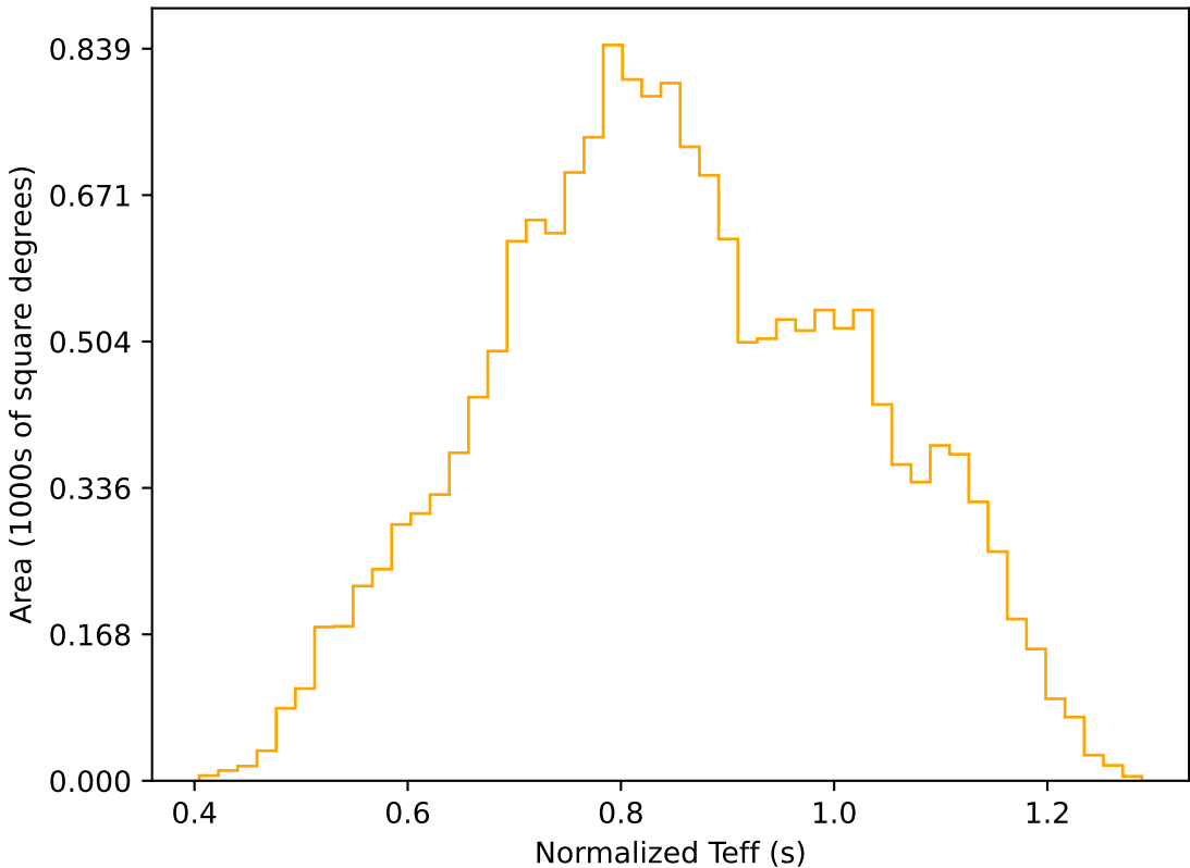
too_elab_r128_d3_gz_v3.4_10yrs WFD r band: Normalized Teff
