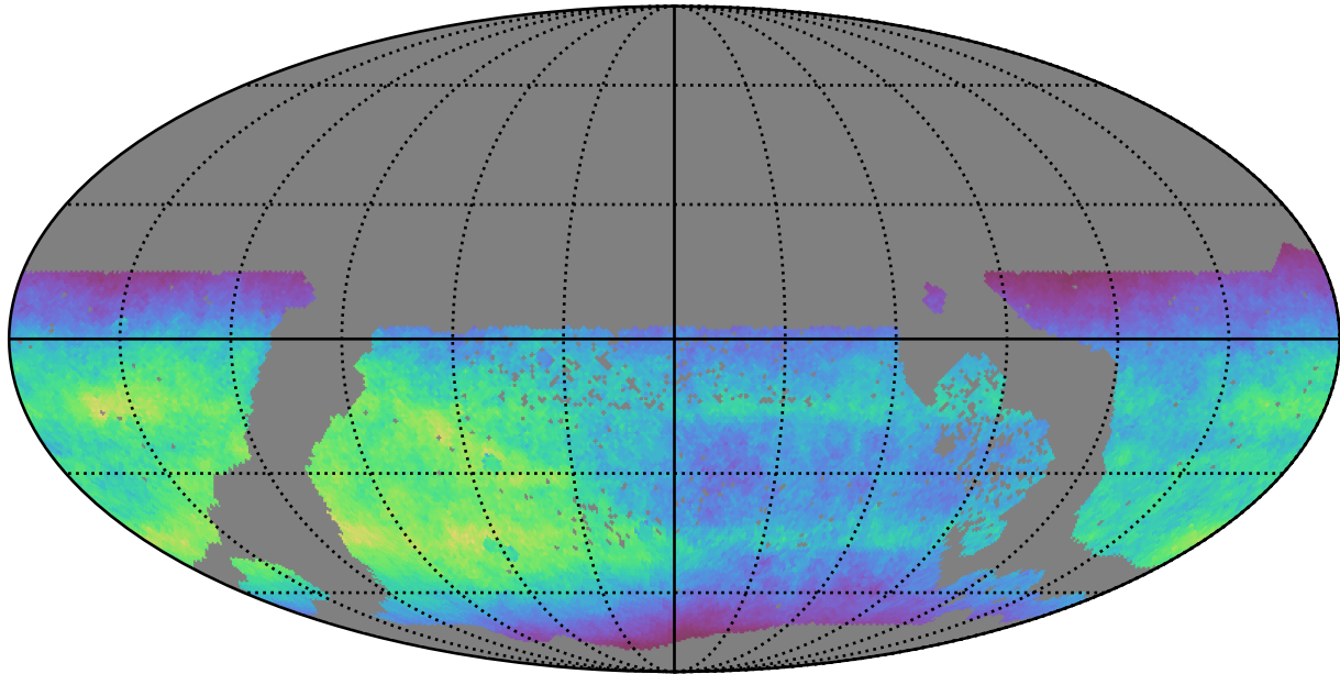
too_elab_r128_d3_gz_v3.4_10yrs WFD i band: Normalized Teff
