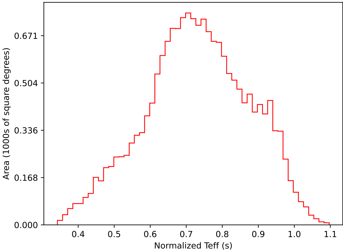
too_elab_r128_d3_gz_v3.4_10yrs WFD i band: Normalized Teff
