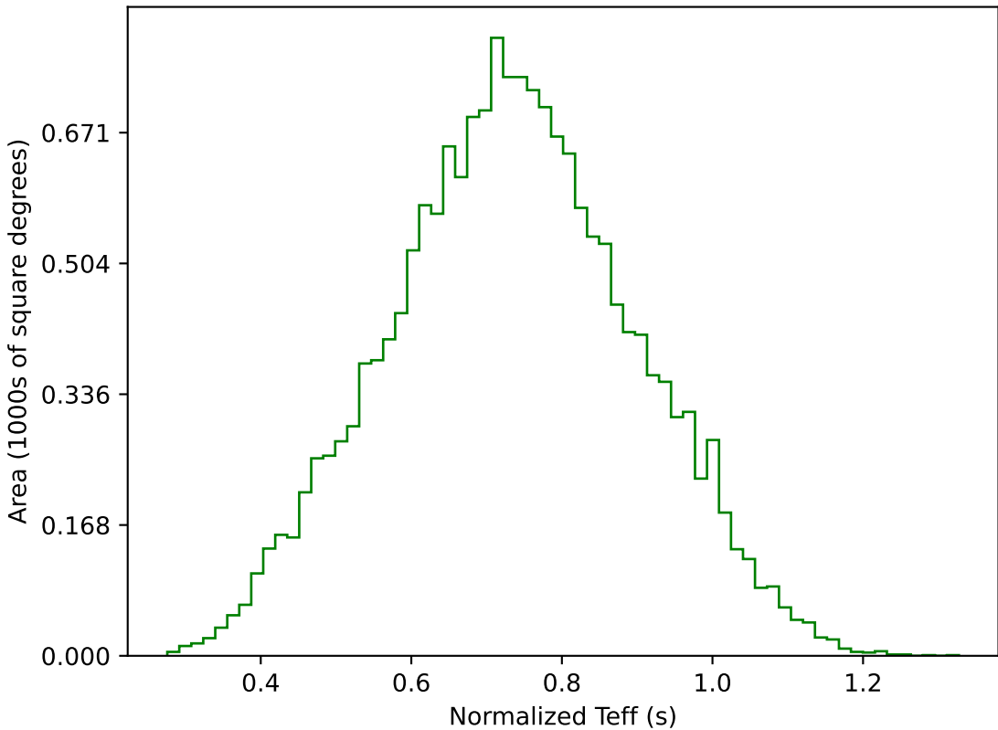
too_elab_r128_d3_gz_v3.4_10yrs WFD g band: Normalized Teff
